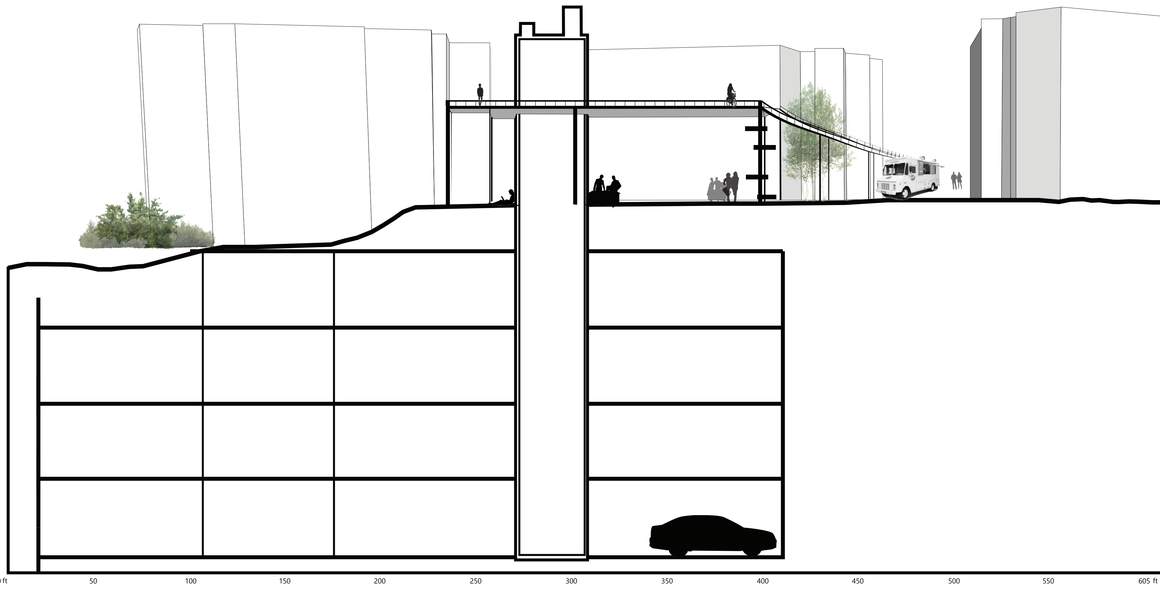
SECTION ELEVATION - ELEVATOR TO KANE CANOPY
